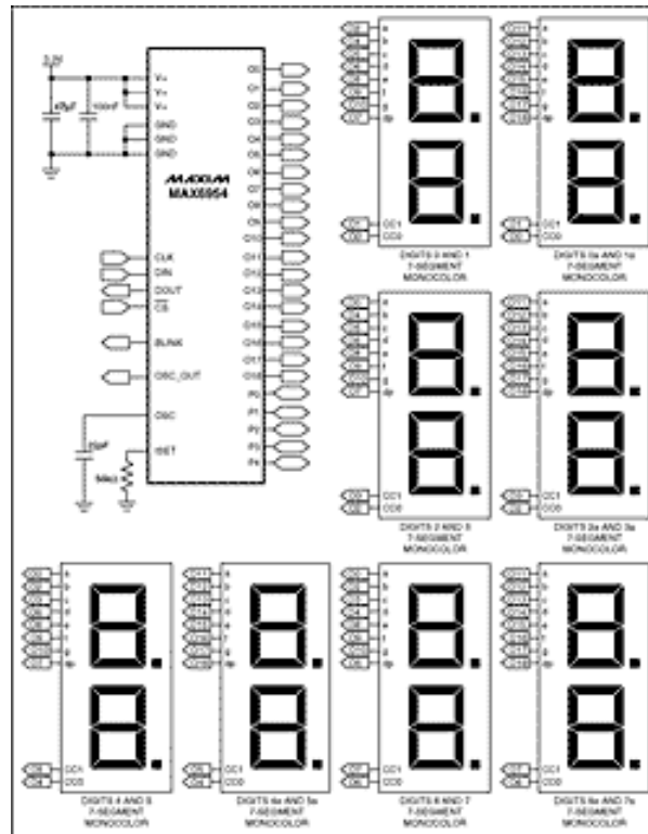
Figure 1. MAX6954 7-Segment Application Circuit
